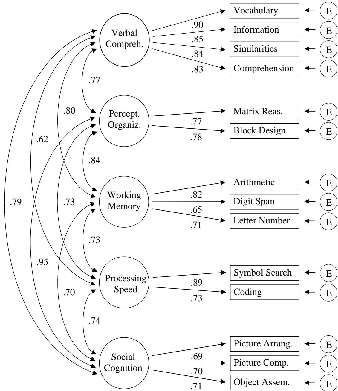
Figure 1. Model M5:PA,PC,OA. Best fitting model for 14 subtests.
